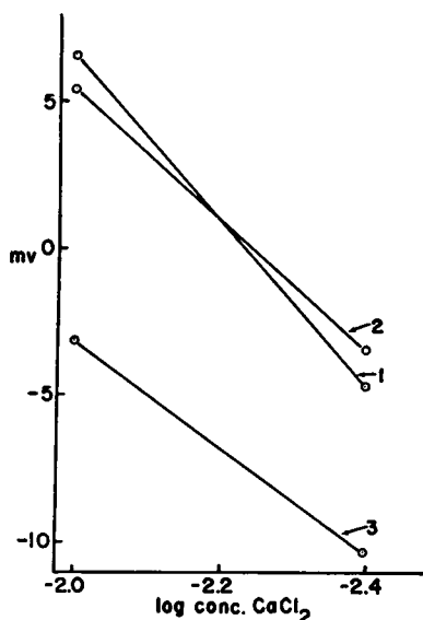
FIGURE 7 Potentials found by measuring a solution, 0.006 M \text{CaCl}_2 , against two solutions, 0.01 and 0.004 M \text{CaCl}_2 , across a PVC + TBP + TTA (1:3:1) membrane. The sign of the potential is that of the 0.006 M \text{CaCl}_2 solution. 1, no perturbing ions present; 2, 0.08 M \text{MgCl}_2 added to all three solutions; 3, 0.08 M \text{NaCl} added only to 0.01 and 0.004 M \text{CaCl}_2 solutions
