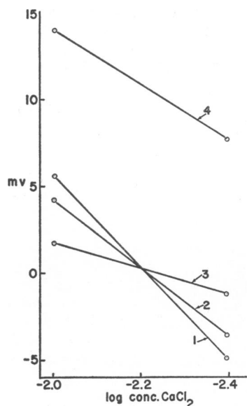
FIGURE 6 Potentials found by measuring a solution, 0.006 M \text{CaCl}_2 , vs two solutions 0.01 and 0.004 M \text{CaCl}_2 across a PVC + TBP (1:3) membrane. The sign of the potential is that of the 0.006 M \text{CaCl}_2 solution. 1, no perturbing ions present; 2, 0.08 M NaCl added to all three solutions; 3, 0.4 M NaCl added to all three solutions; 4, 0.08 M NaCl added only to 0.01 and 0.004 M \text{CaCl}_2 solutions.
